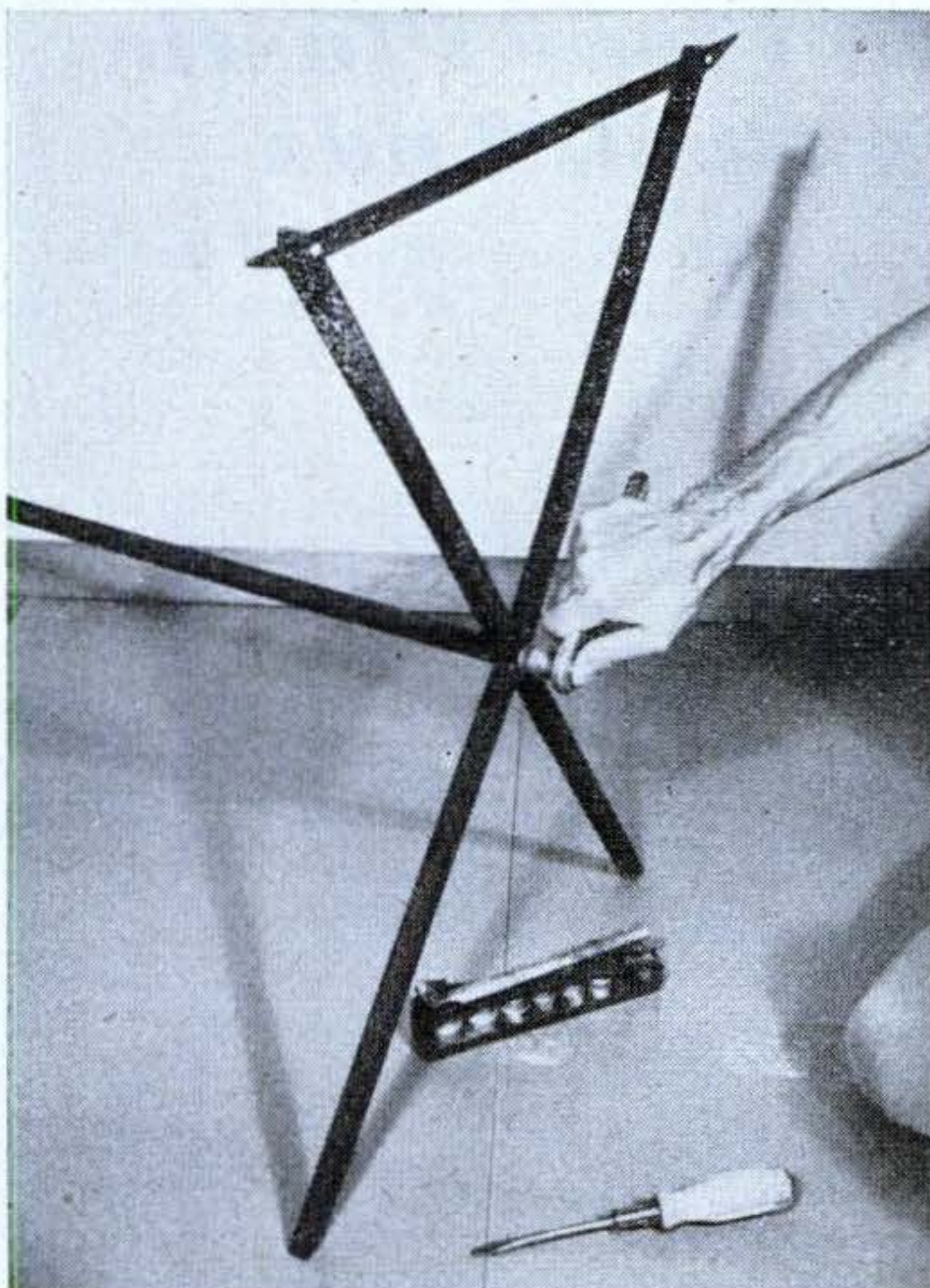
Two bolts hold the top rail. The stretcher is secured with a bolt through the half-lap joint.
